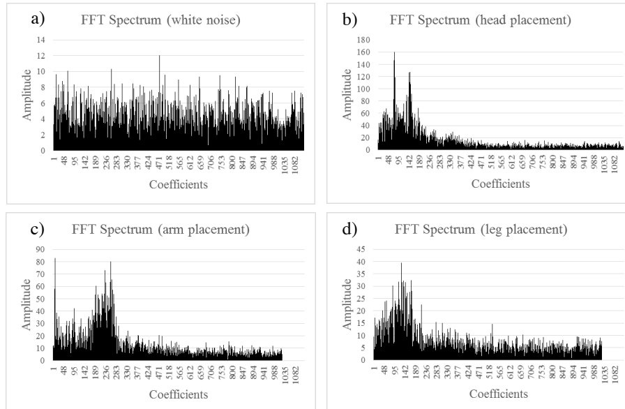
Fig. 2 Frequency spectrum of the gyroscope sensor data. Subfigure (a) shows a white noise. In this measurement setup the sensor was lying on a table. Subfigure (b) shows the frequency spectrum for a head placement. Subfigure (c) shows the frequency spectrum for an arm placement. Subfigure (d) shows the frequency for a leg placement.
